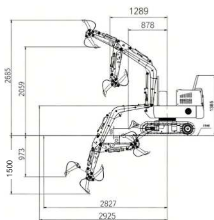
Working range
